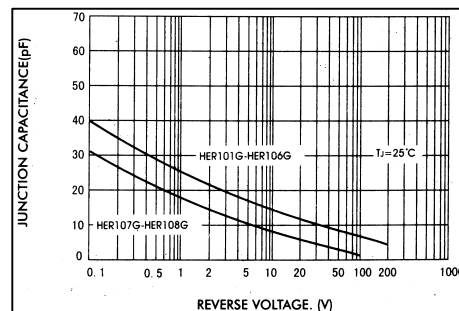
FIG.6-TYPICAL JUNCTION CAPACITANCE
