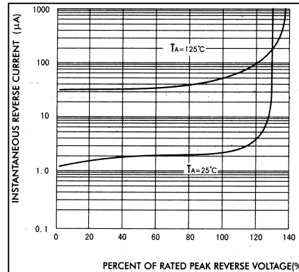
FIG.4-TYPICAL REVERSE CHARACTERISTICS
